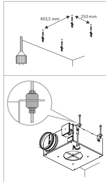
Mounting using four holders
